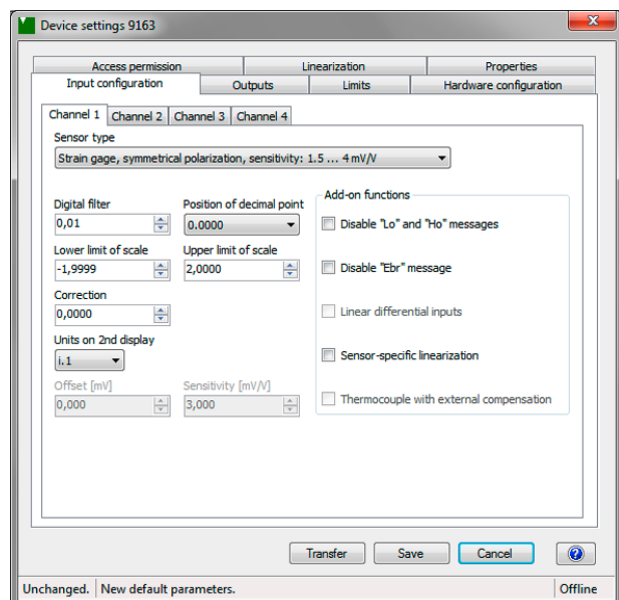
Instrument parameterization
